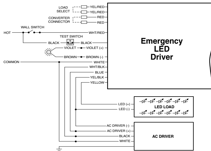
FIG A TWO (2) WIRE INTEGRATED TEST SWITCH
