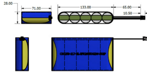
BSL20B6 Battery (mm)
