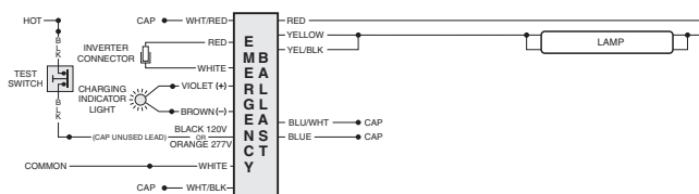
FIG J ONE (1) 32-215 W LAMP WITHOUT AC BALLAST
