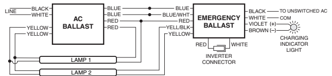
FIG B TWO (2) LAMP RAPID START BALLAST (2'-4' T8, T10, T12 LAMPS ONLY)
